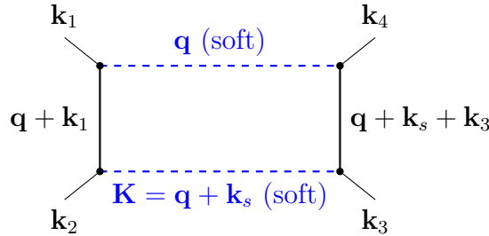
Figure 1: All momentum labels are vectors. Dashed lines select the double-soft region; solid internal lines retain complete hard time dependence.
